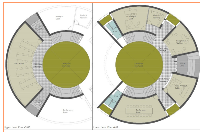
Plan of Admin Block
